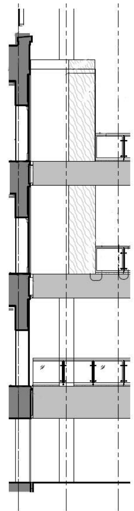
Figure 6 | Atrium - Elevation
